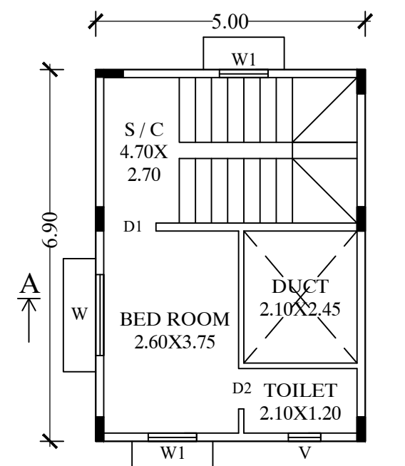
PROPOSED TYPICAL FIRST & SECOND FLOOR PLAN
